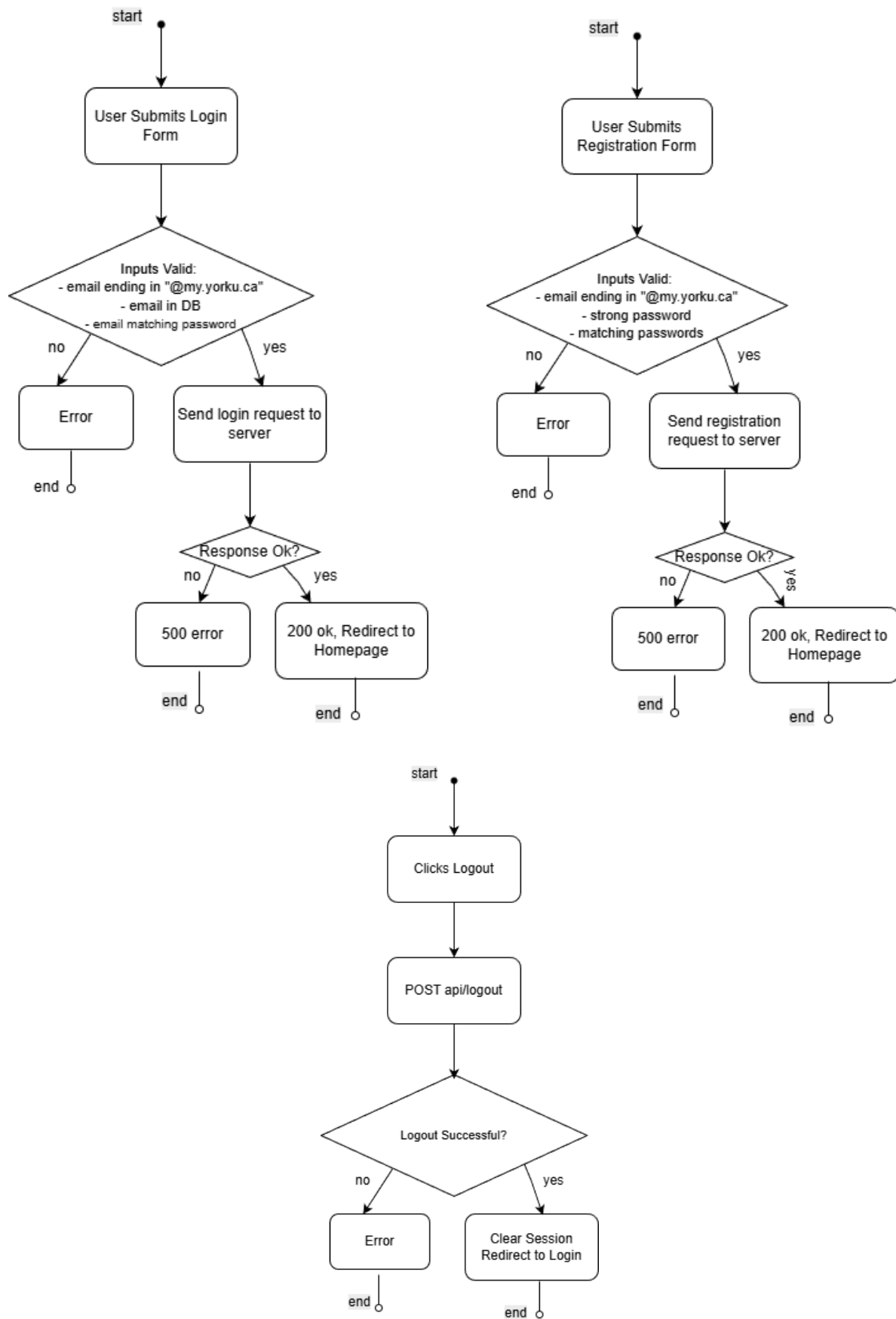
Registration, Login and Logout Diagrams:
